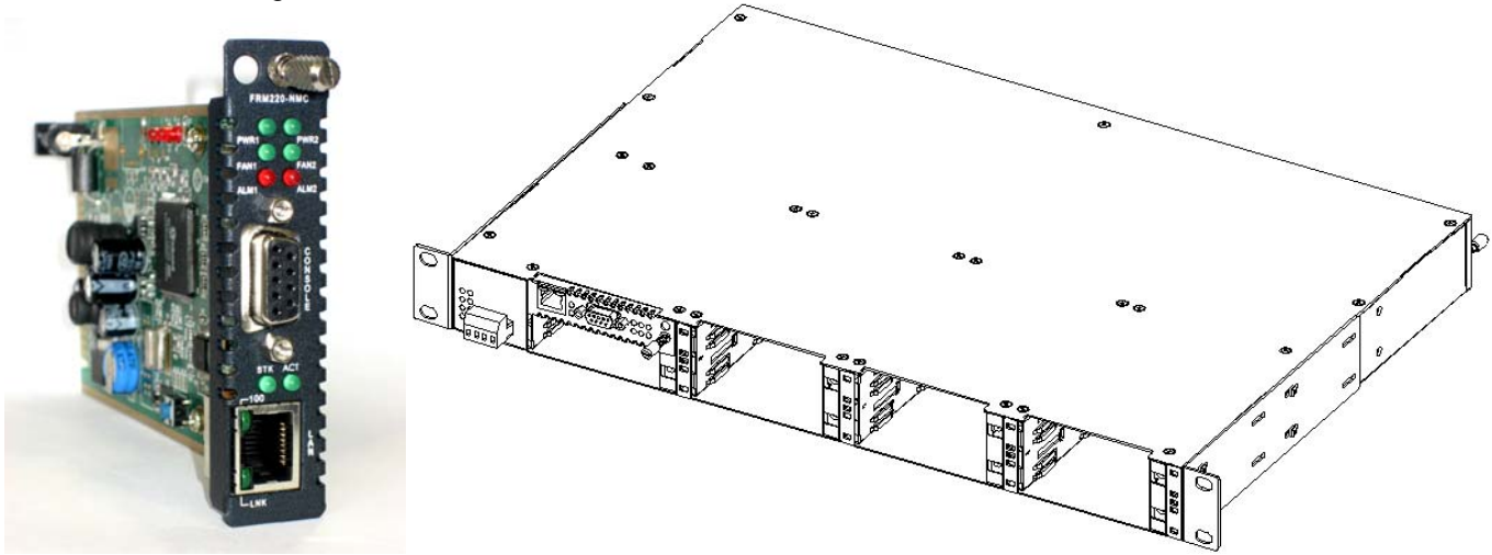
Figure 2-7 NMC removal/replacement in slot number 1
