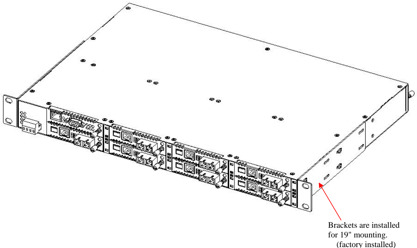
Figure 2-1 Standard 19" Rack-Mount Installation of CH08 Unit requires 1RU space
