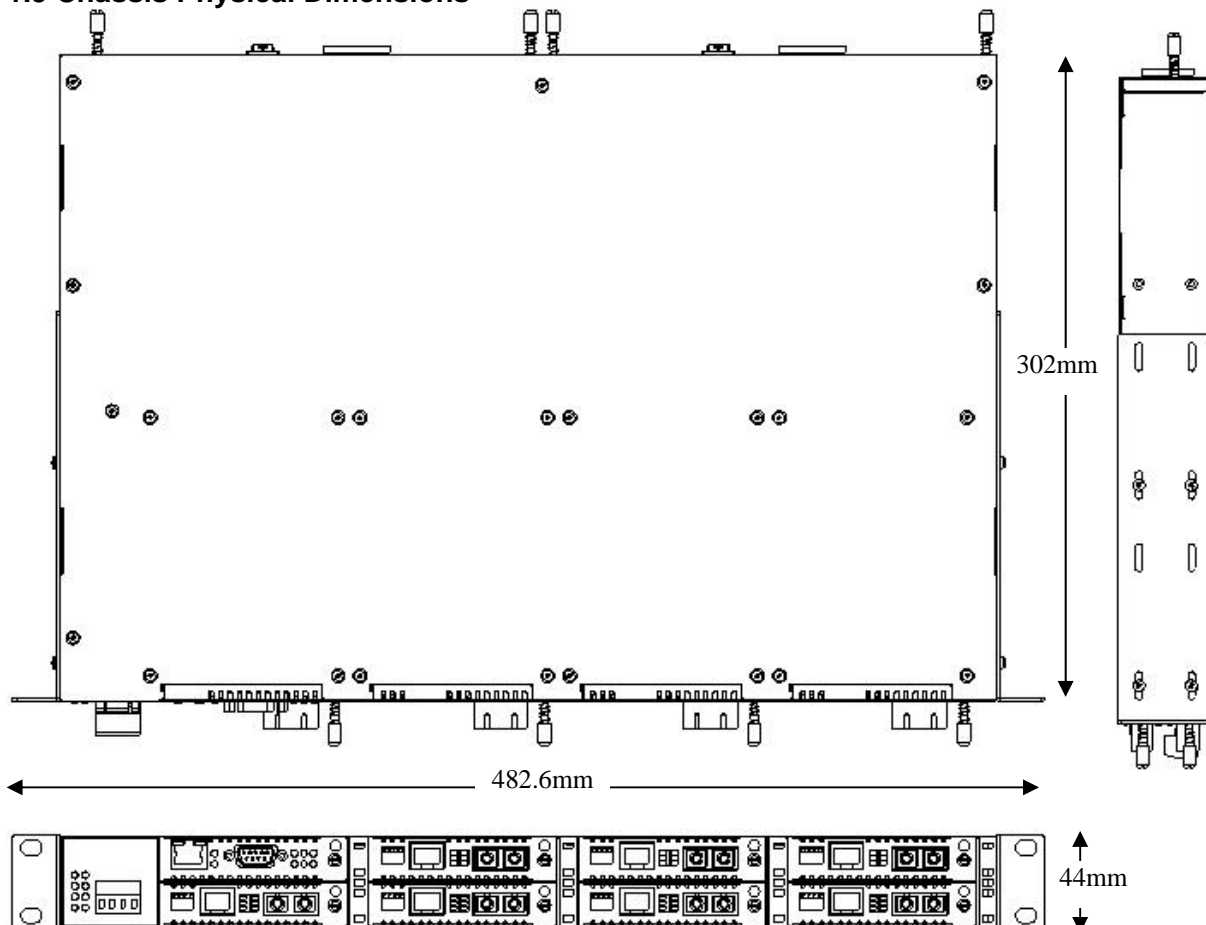
Figure 1-4 Chassis Dimensions, in millimeters
