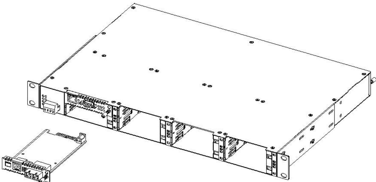
Figure 2-8 Line card removal/replacement
