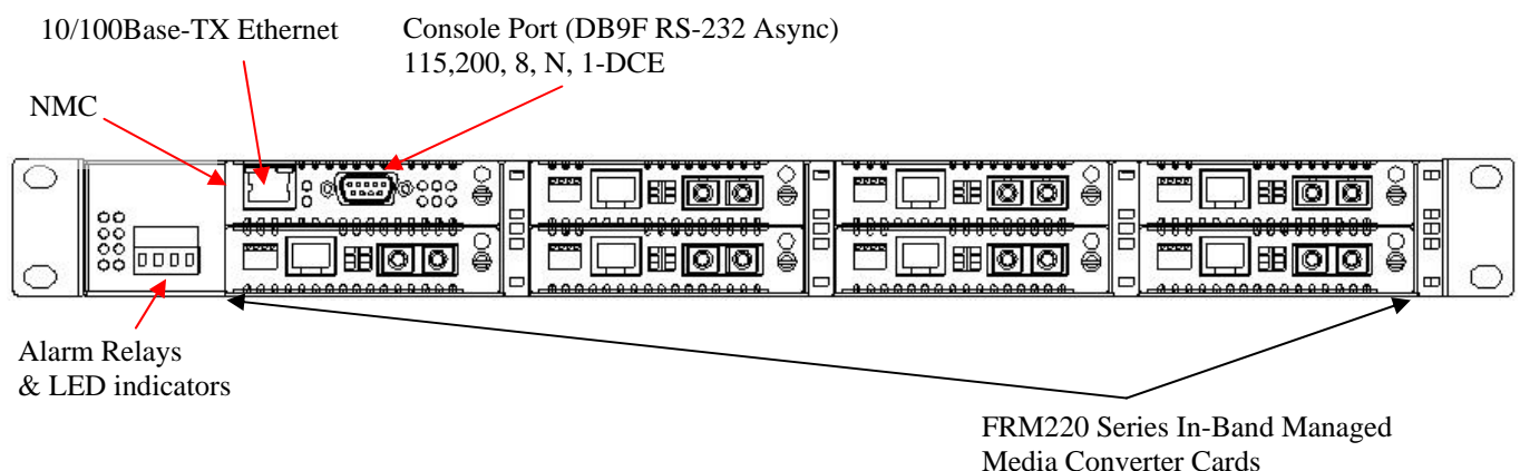
Figure 1-1 Chassis Front View
