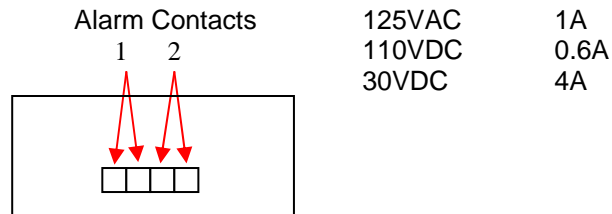
Figure 2-5 Alarm Relay Contacts
