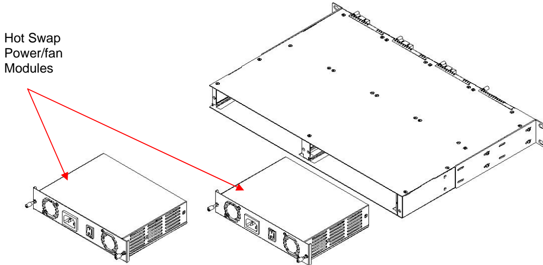
Figure 2-2 Power Modules for CH08
