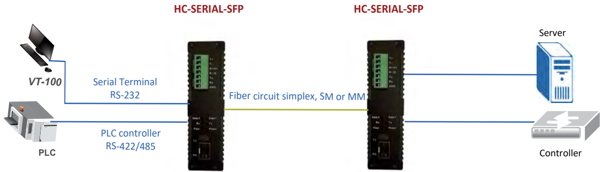
HC-SERIAL-SFP RS-232/RS-485 extension over fiber application
