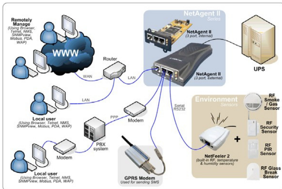
Connect to SNMP-2PV2
